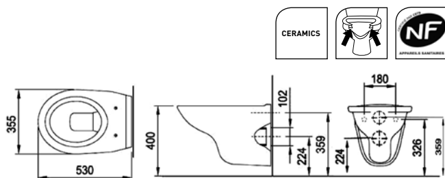
HANGTOILET 530 MM WC SUSPENDU 530 MM WAND-WC 530 MM
