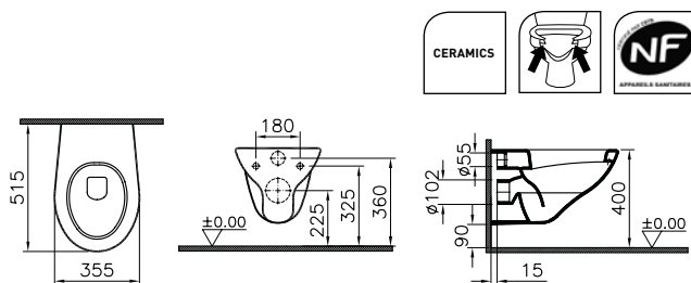
HANGTOILET 515 MM WC SUSPENDU 515 MM WAND-WC 515 MM
