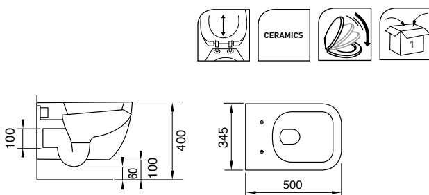
HANGWC PACK PACK CUVETTE SUSPENDUE PACK WAND-WC
