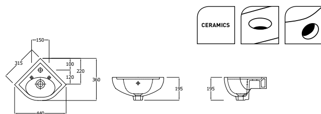
HOEKHANDENWASSER 440 X 360 MM LAVE-MAINS ANGLE 440 X 360 MM ECKHANDWASCHBECKEN 440 X 360 MM
