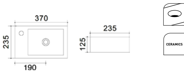
HANDENWASSER LINKS 370 X 235 MM LAVE-MAINS GAUCHE 370 X 235 MM HANDWASCHBECKEN LINKS 370 X 235 MM
