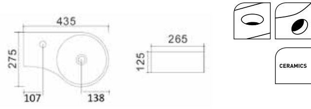
HANDENWASSER LINKS 435 X 275 MM LAVE-MAINS GAUCHE 435 X 275 MM HANDWASCHBECKEN LINKS 435 X 275 MM
