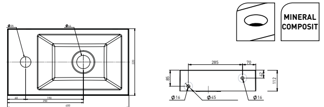
HANDENWASSER LINKS 400 X 220 MM LAVE-MAINS GAUCHE 400 X 220 MM HANDWASCHBECKEN LINKS 400 X 220 MM
